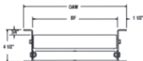
Single roller design
